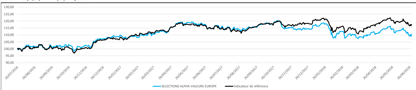
Performance (26/07/2016 - 29/06/2018) - Base 100
